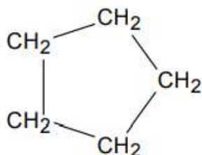
cyclopentane
